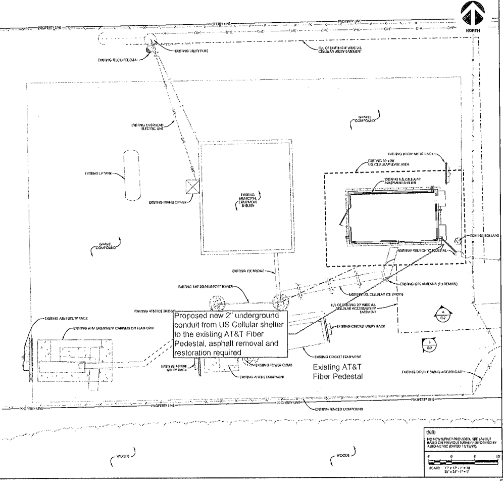
Existing AT&T Fiber Pedestal (A) COMPOUND OVERVIEW (LOOKING NORTH)
